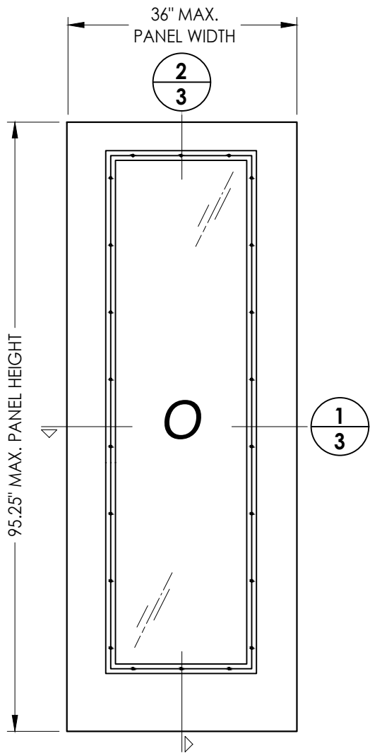
50 SIDELITE PANEL
